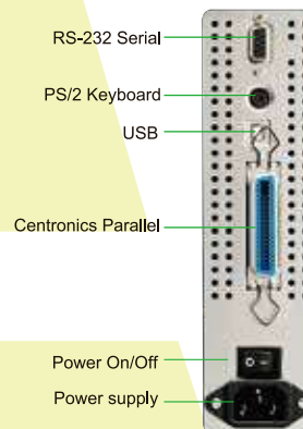
Communication interface
